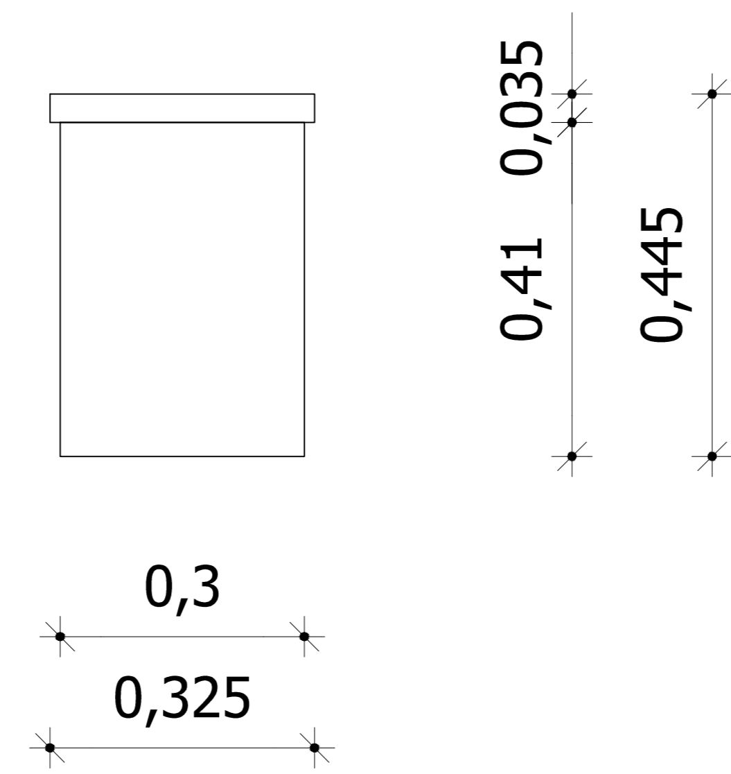
Side View
