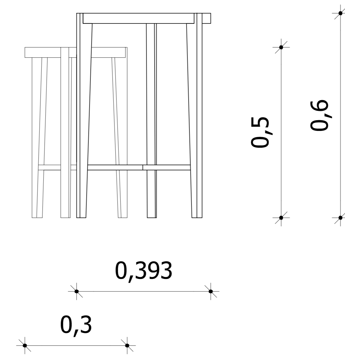
Side View
