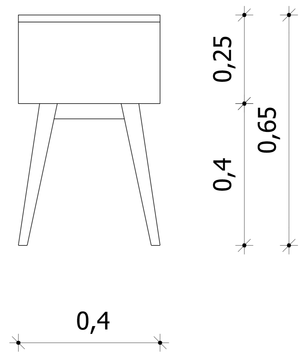
Side View
